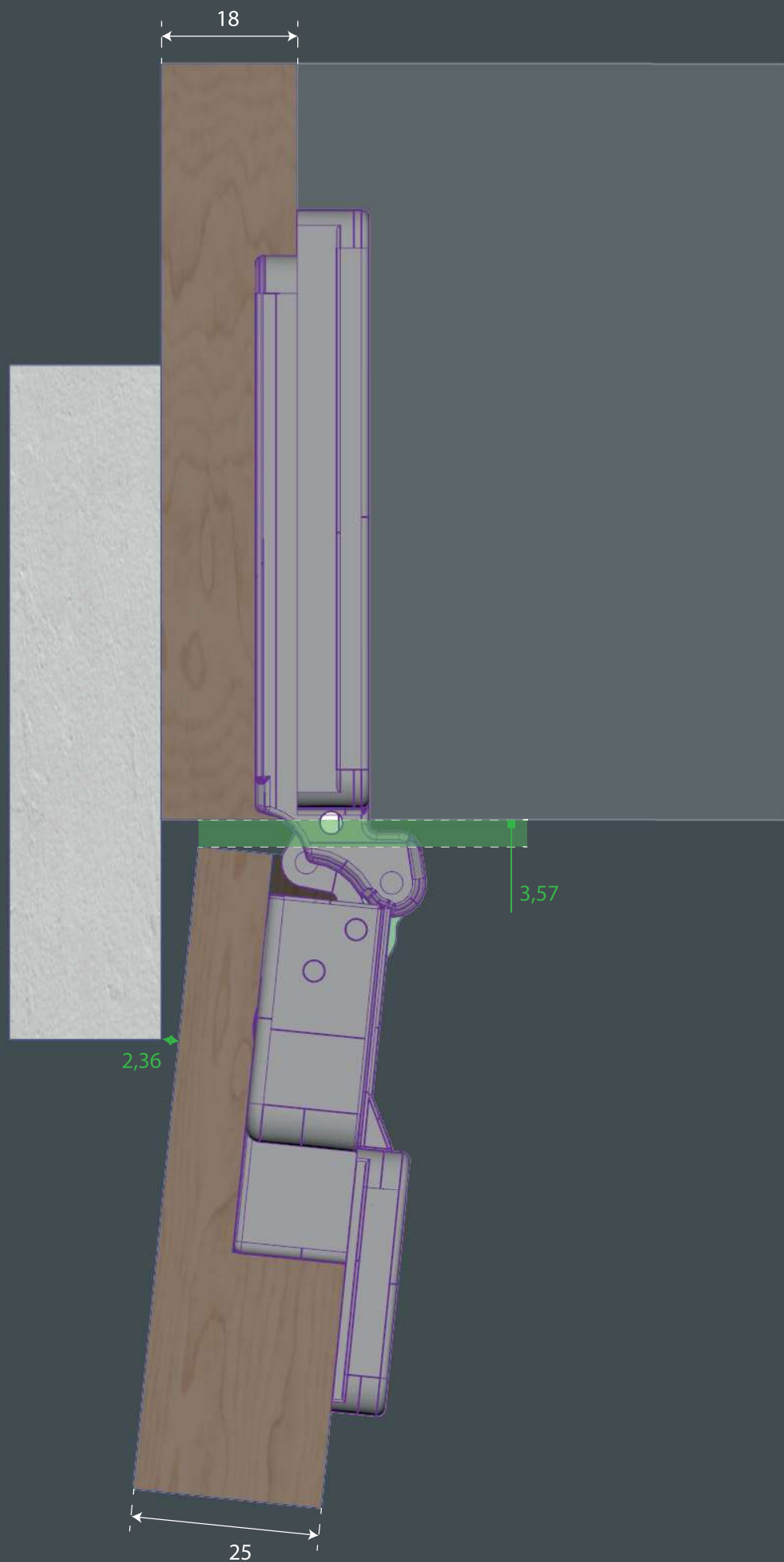
25mm door , 18mm side-board ( A=53mm ) - v03
