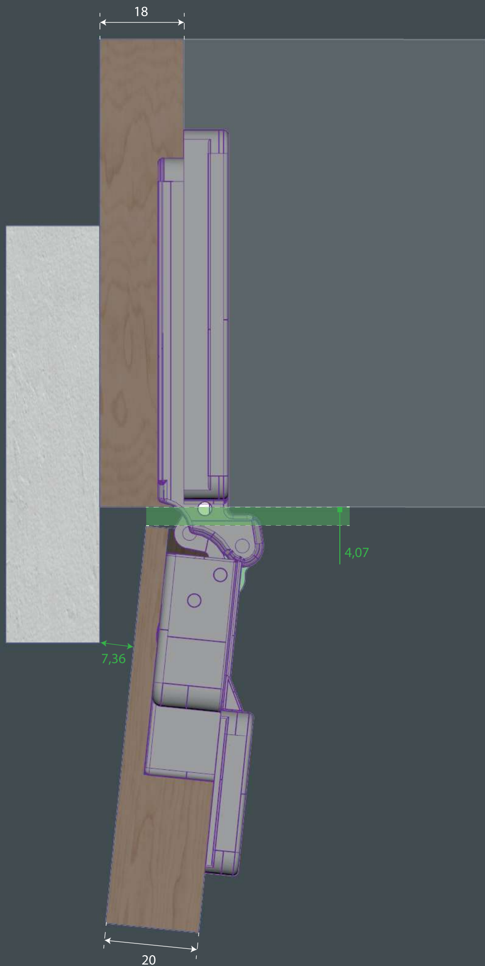
20mm door , 18mm side-board ( A=53mm )- v03
