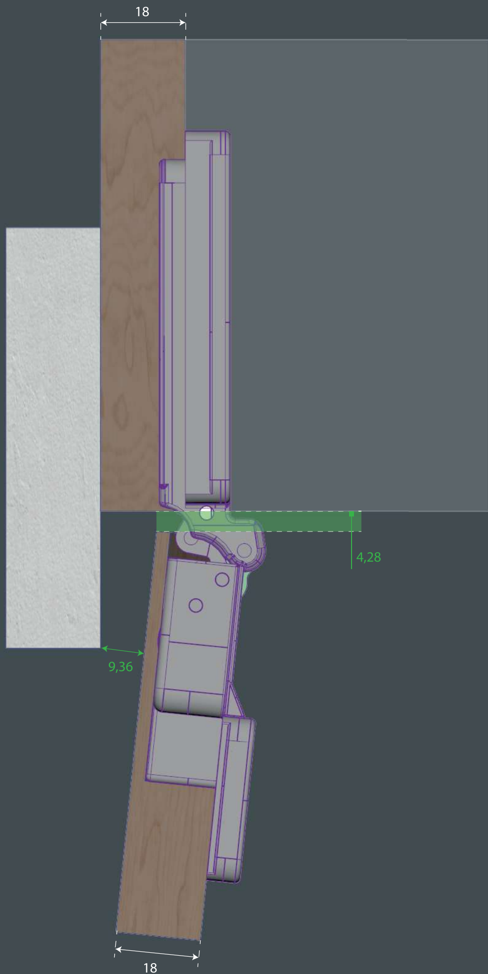
18mm door , 18mm side-board ( A=53mm ) - v03
